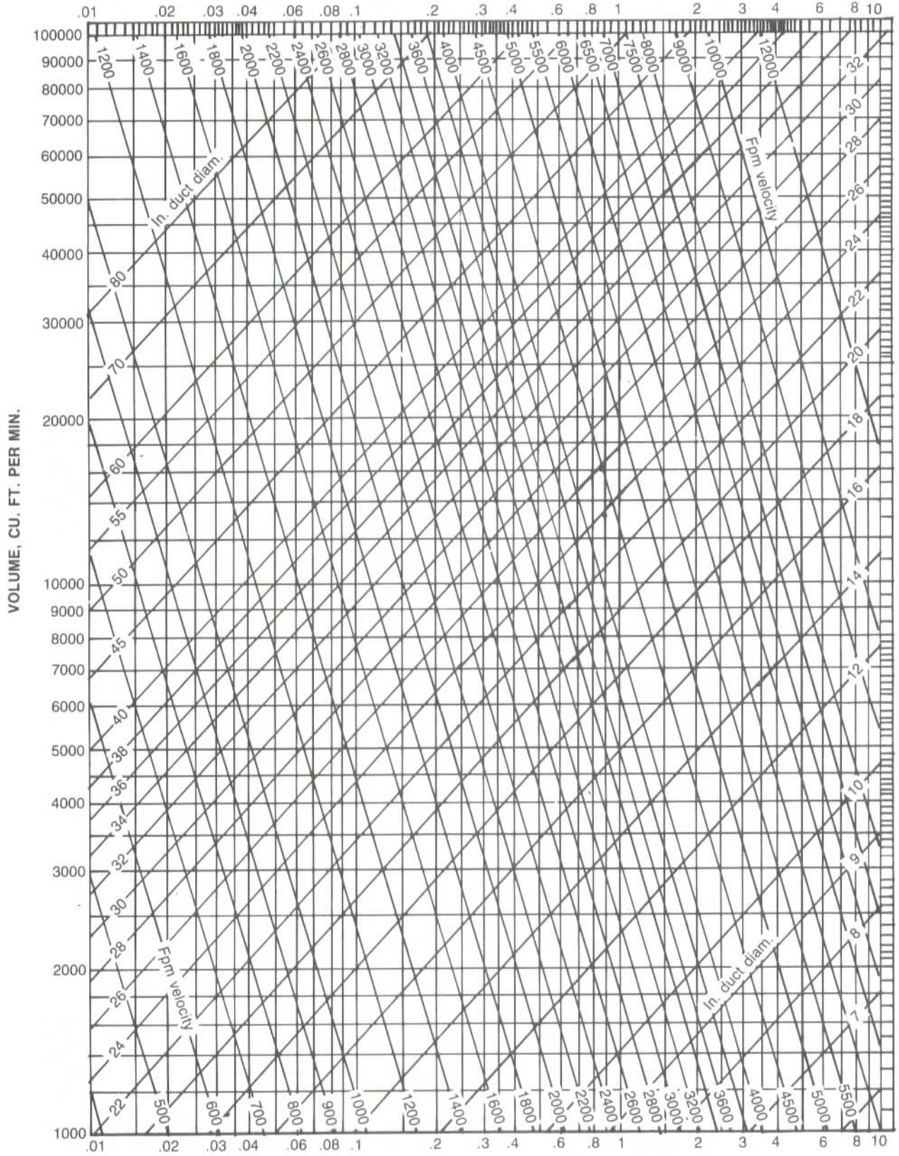
FRICTION OF AIR FOR VOLUMES OF 1000 to 100000 CFM. 7 TO 80" ID
